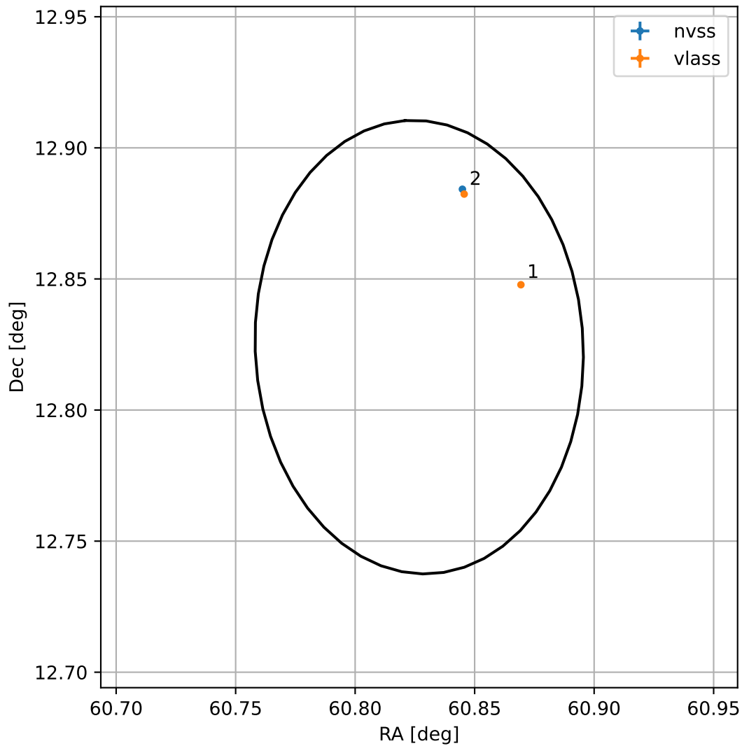
4FGL J0403.3+1249
