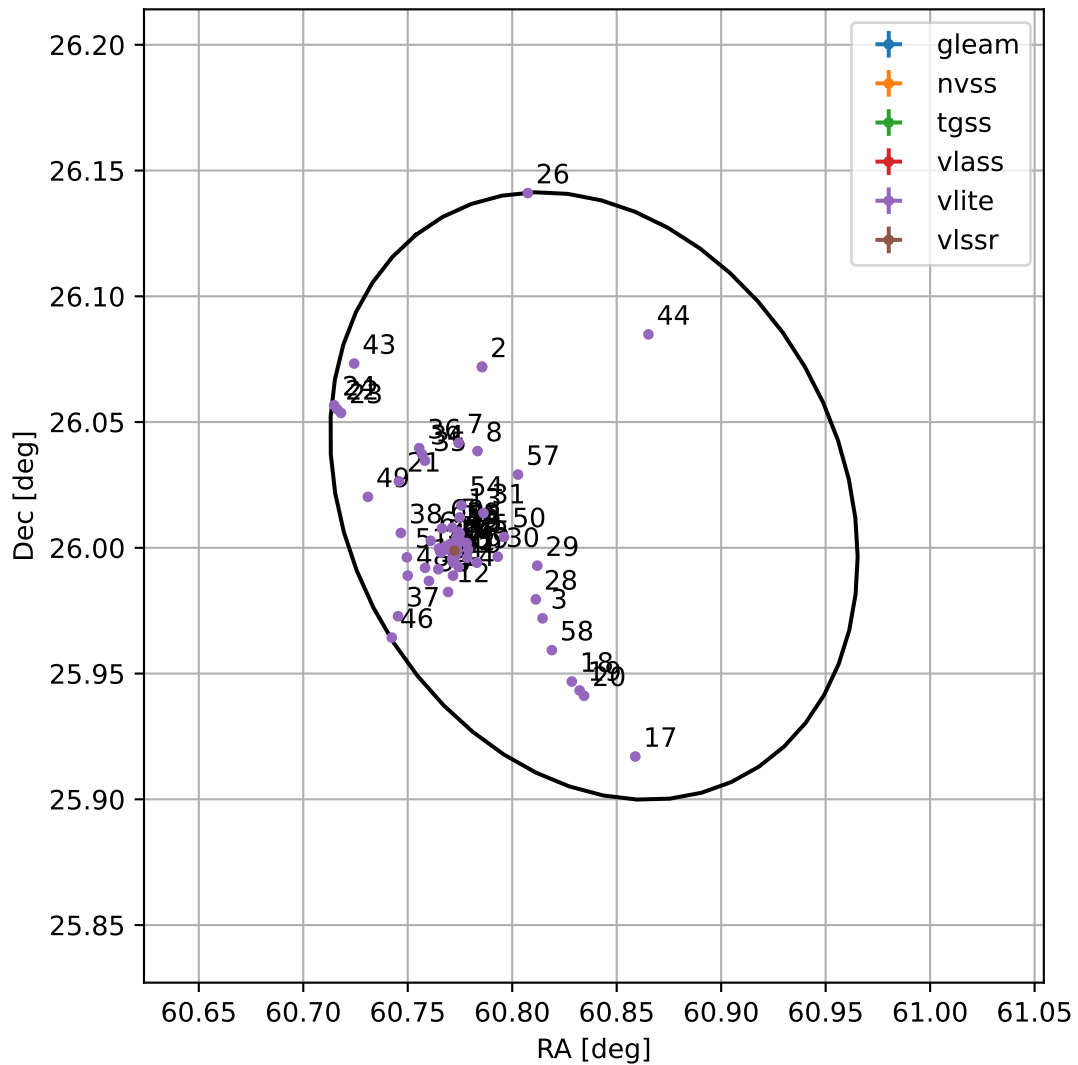
4FGL J0403.3+2601
