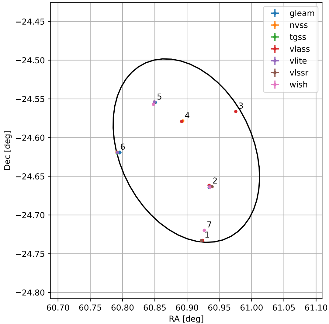
4FGL J0403.5-2437
