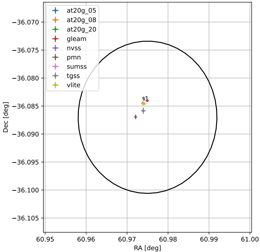
4FGL J0403.9-3605
