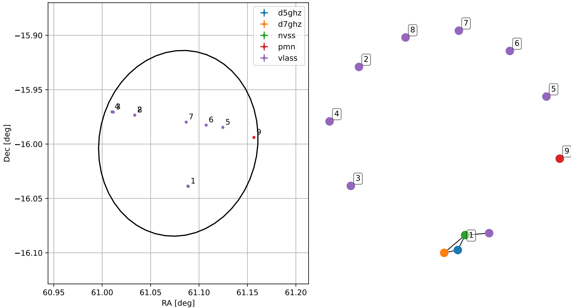
4FGL J0404.3-1559
