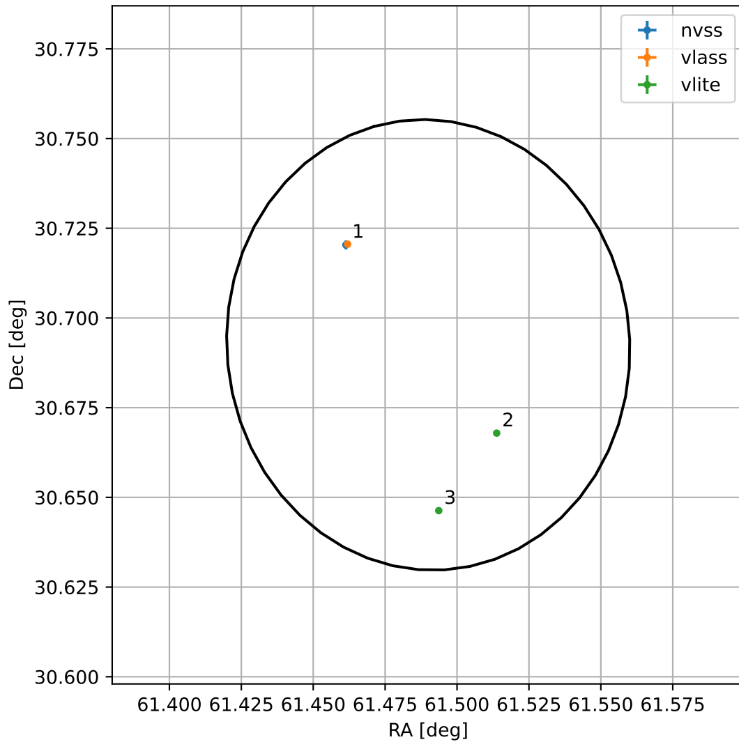
4FGL J0405.9+3041
