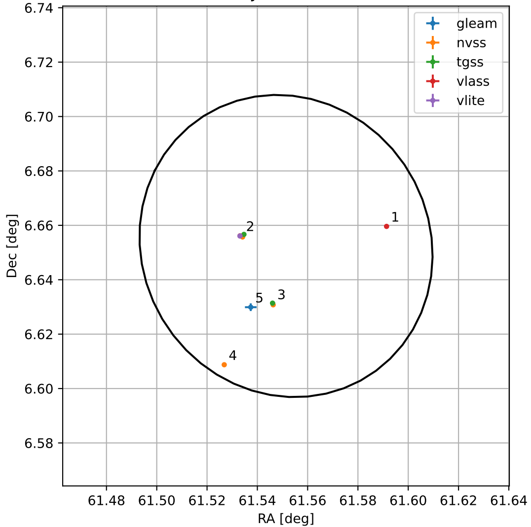
4FGL J0406.2+0639
