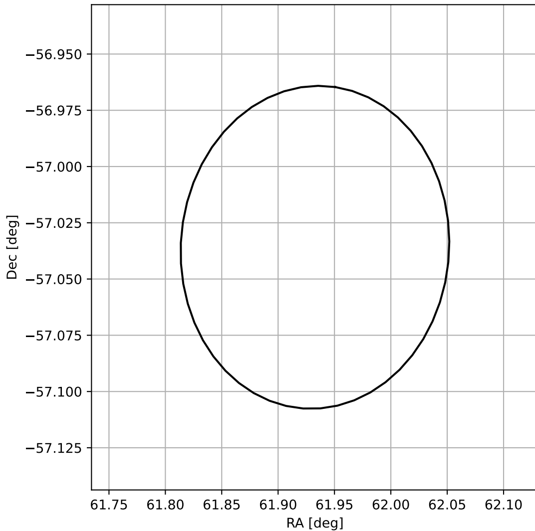
4FGL J0407.7-5702
