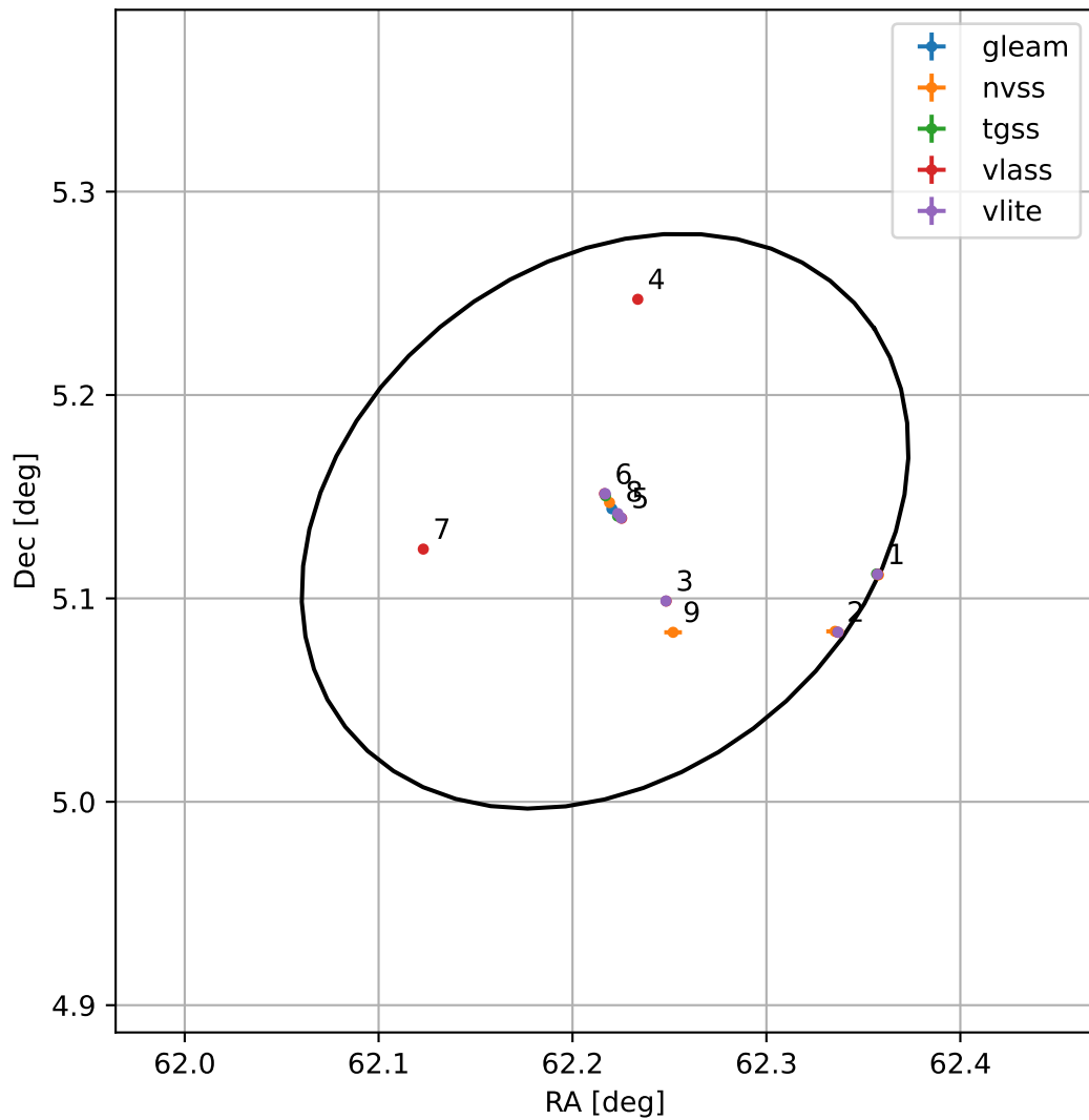
4FGL J0408.8+0508
