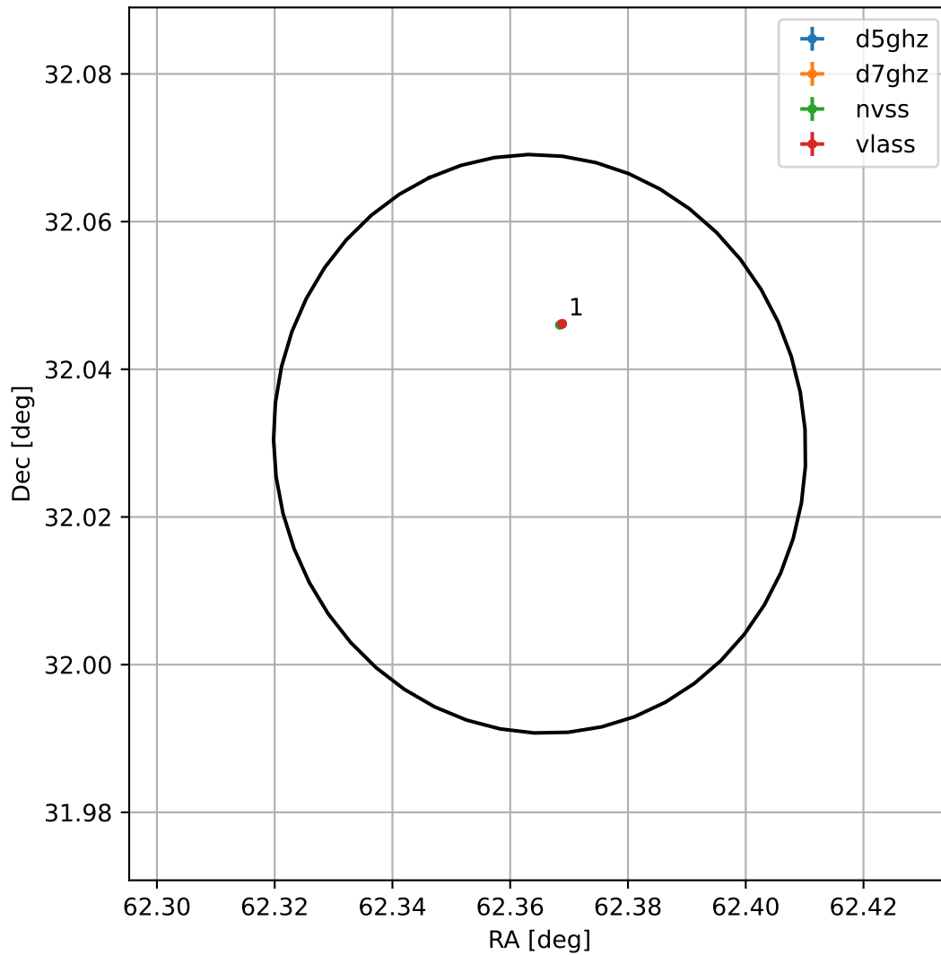
4FGL J0409.4+3201
