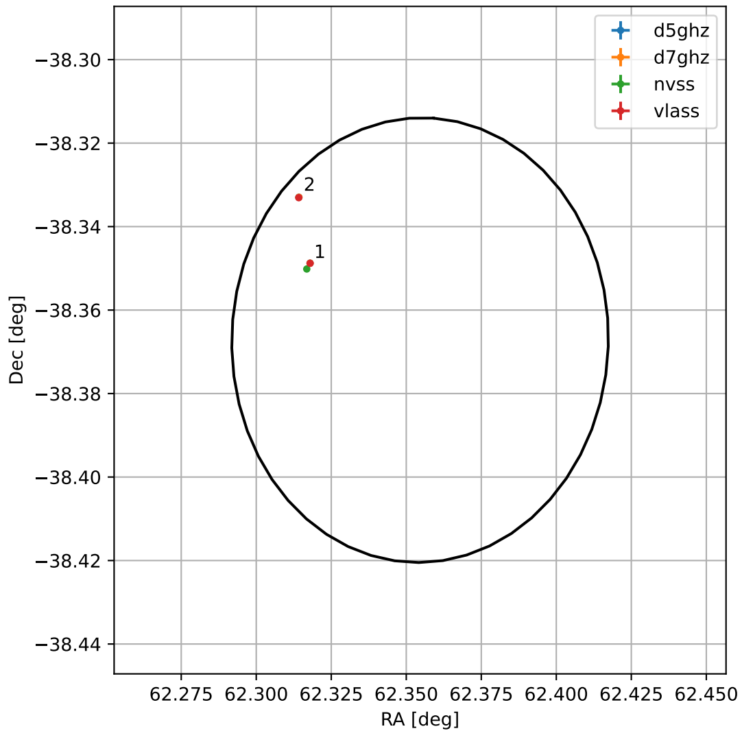
4FGL J0409.4-3822
