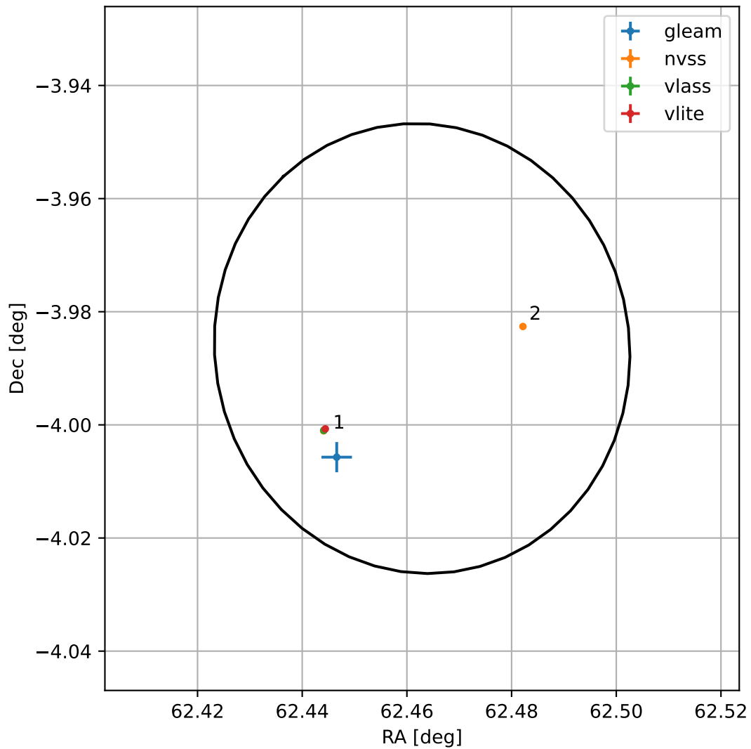
4FGL J0409.8-0359
