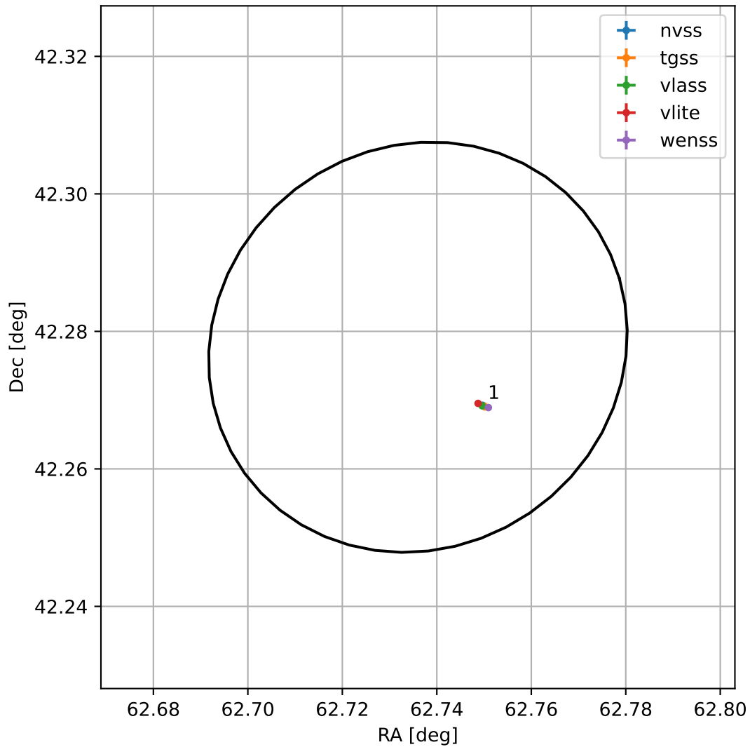
4FGL J0410.9+4216
