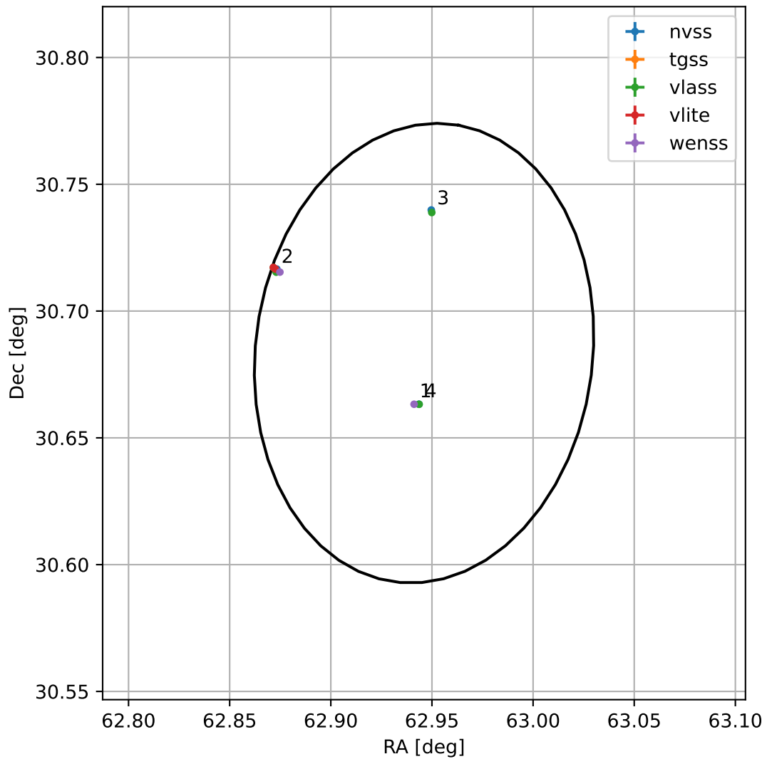
4FGL J0411.7+3041
