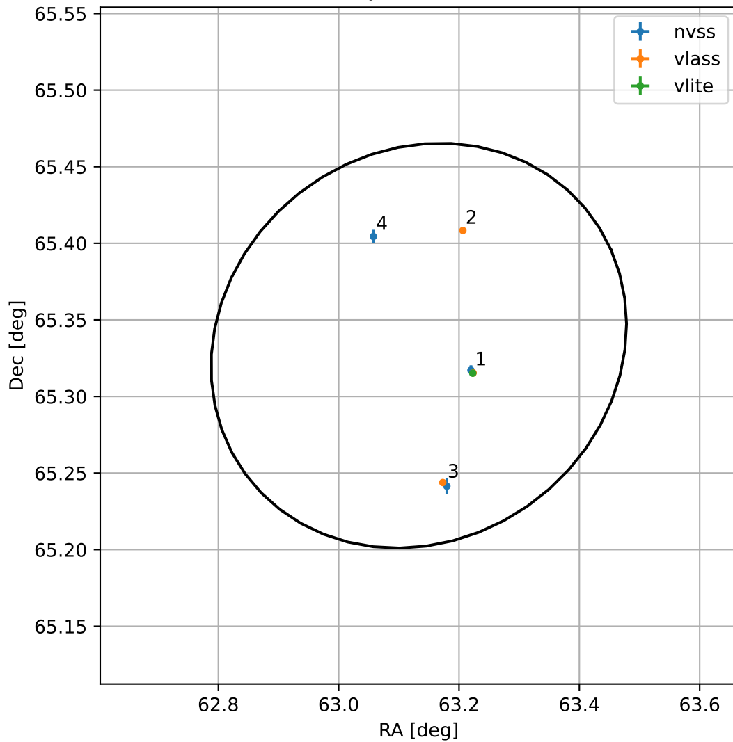
4FGL J0412.5+6519
