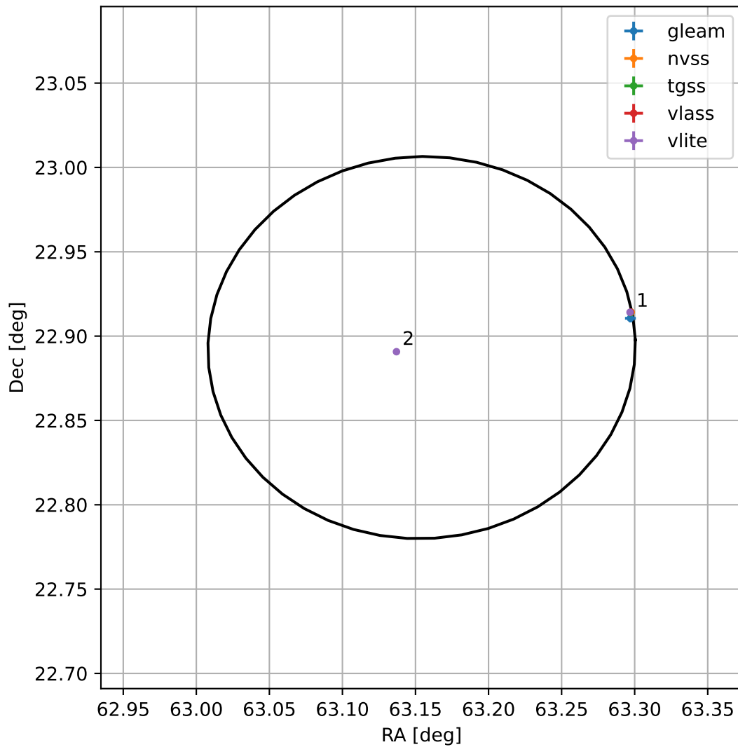
4FGL J0412.6+2253
