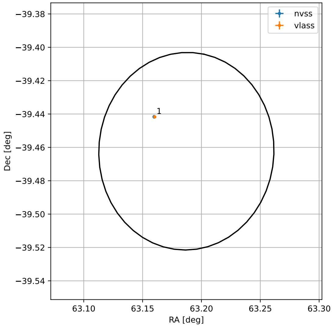
4FGL J0412.7-3927
