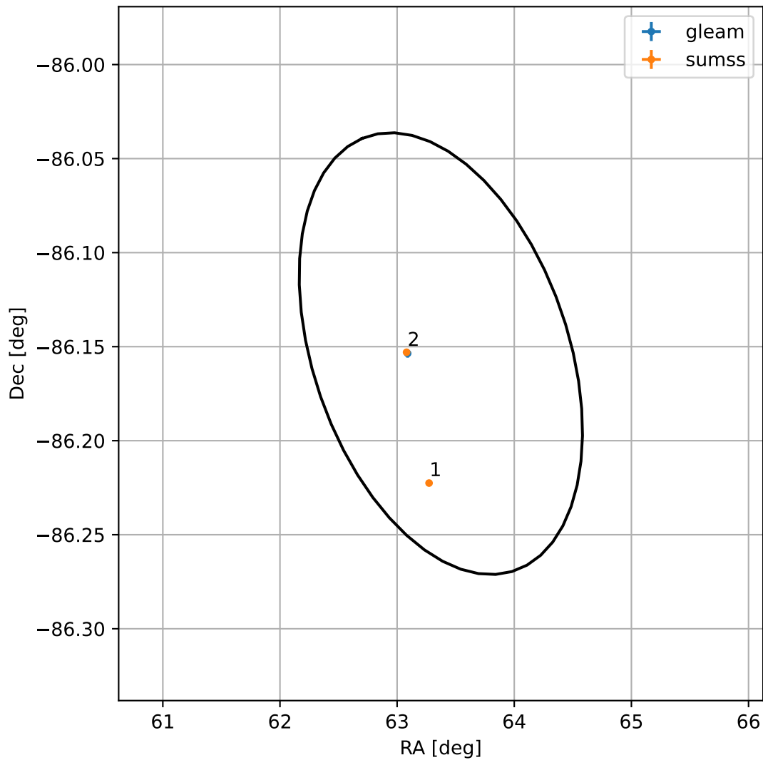
4FGL J0413.4-8609
