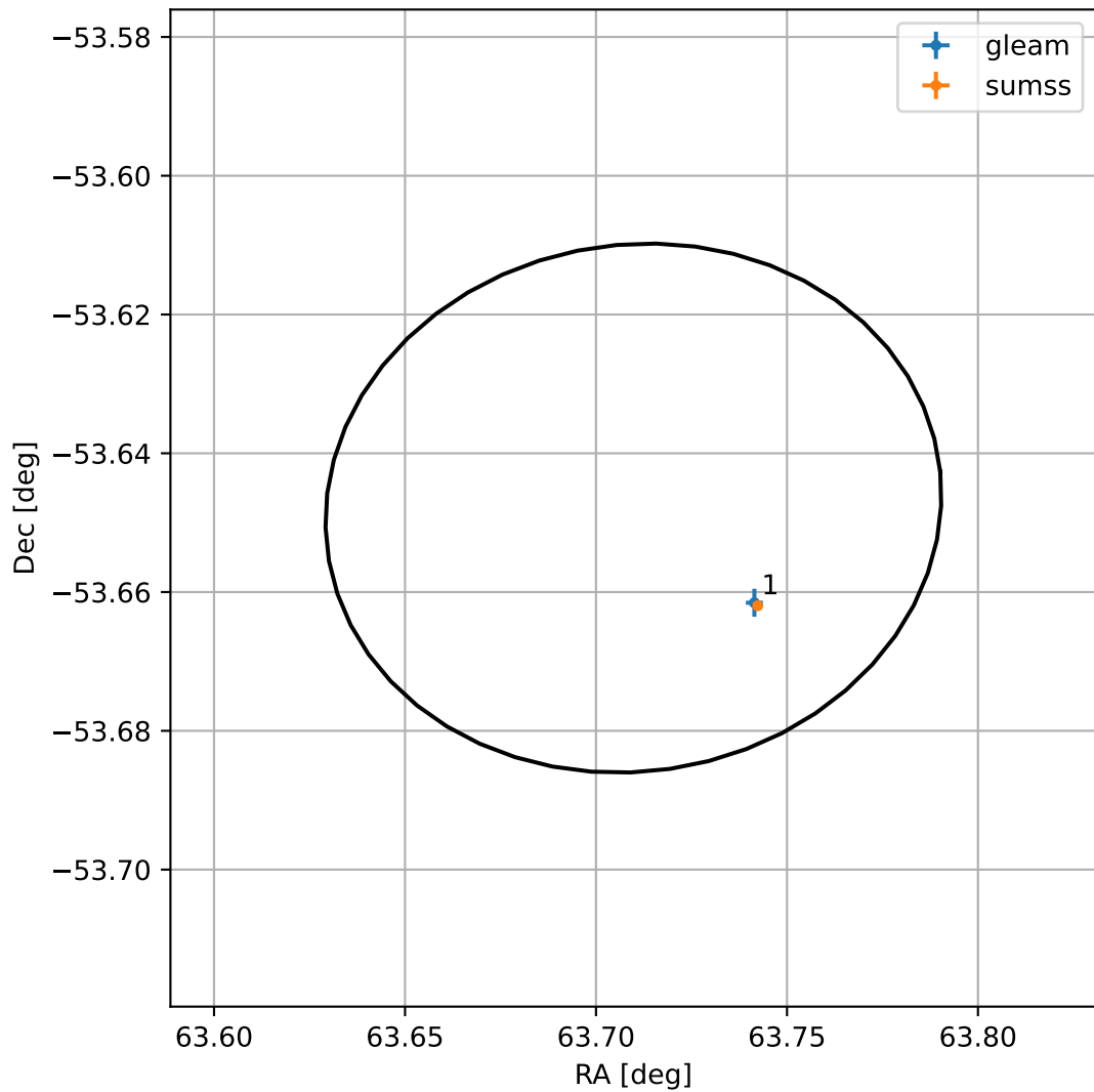
4FGL J0414.8-5338
