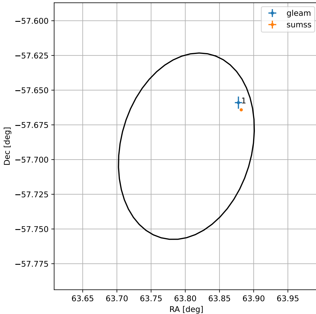
4FGL J0415.2-5741
