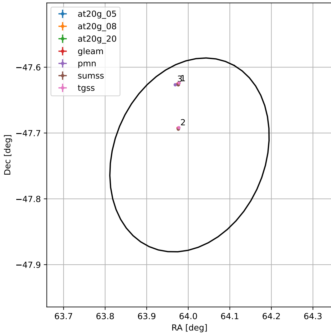
4FGL J0416.0-4743
