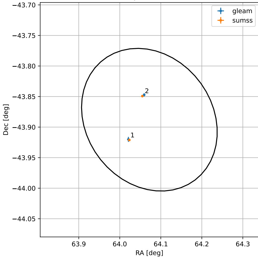
4FGL J0416.2-4353
