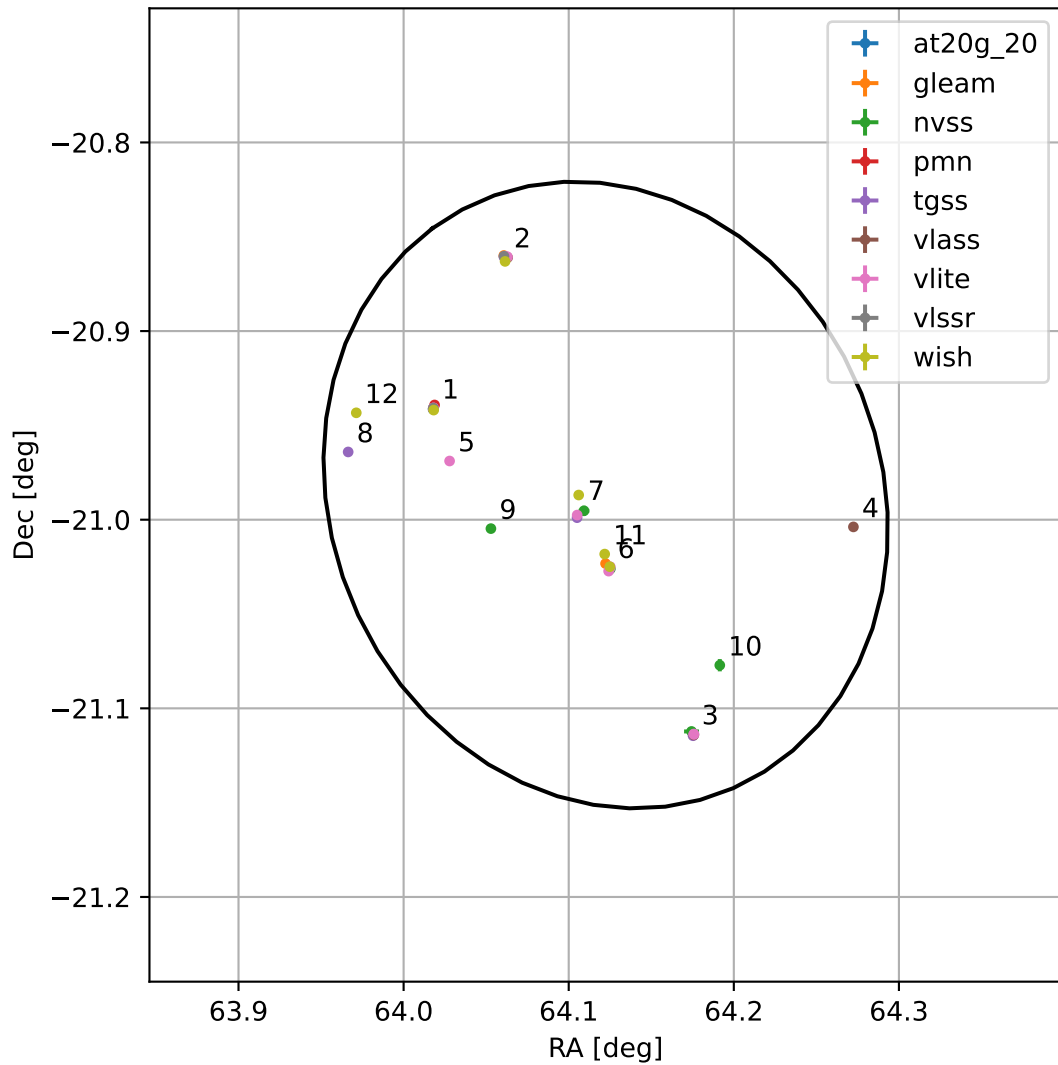
4FGL J0416.4-2059
