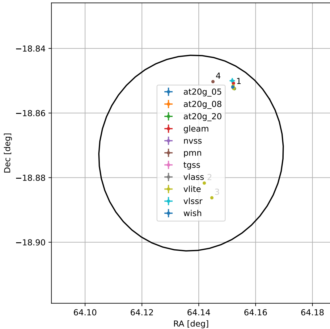
4FGL J0416.5-1852
