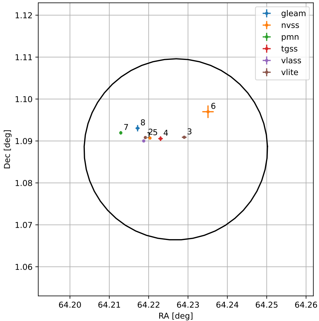
4FGL J0416.9+0105
