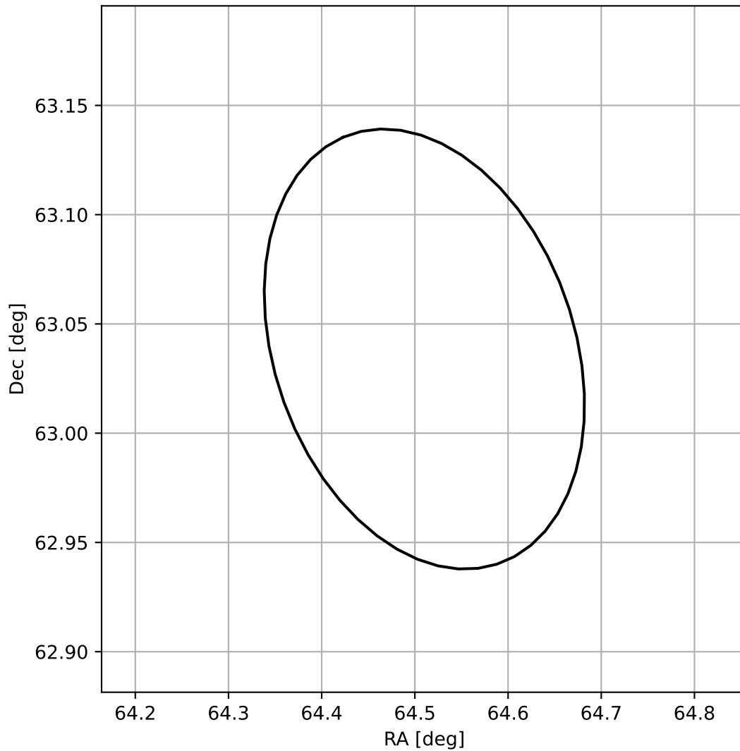
4FGL J0418.0+6302
