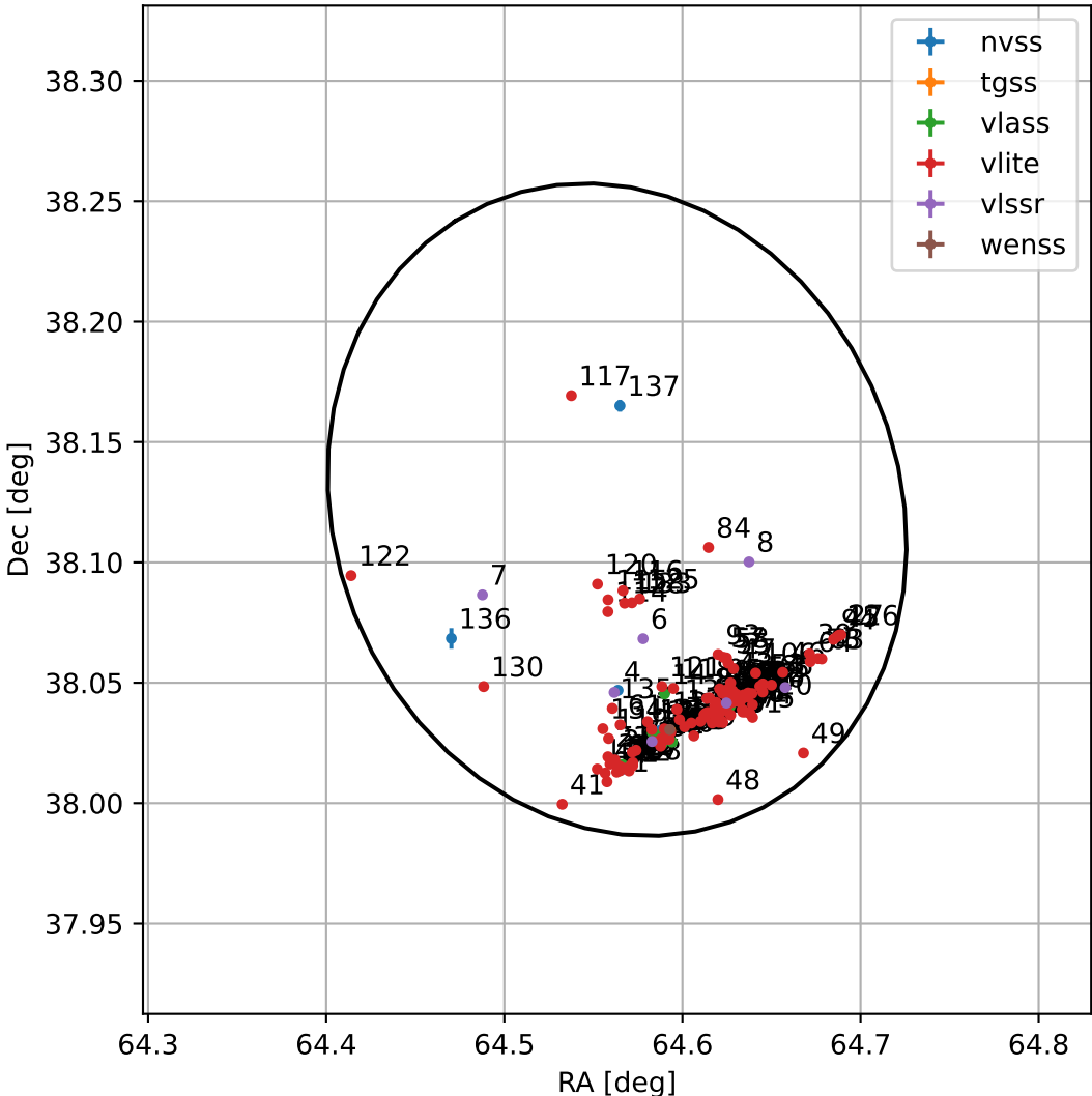
4FGL J0418.2+3807
