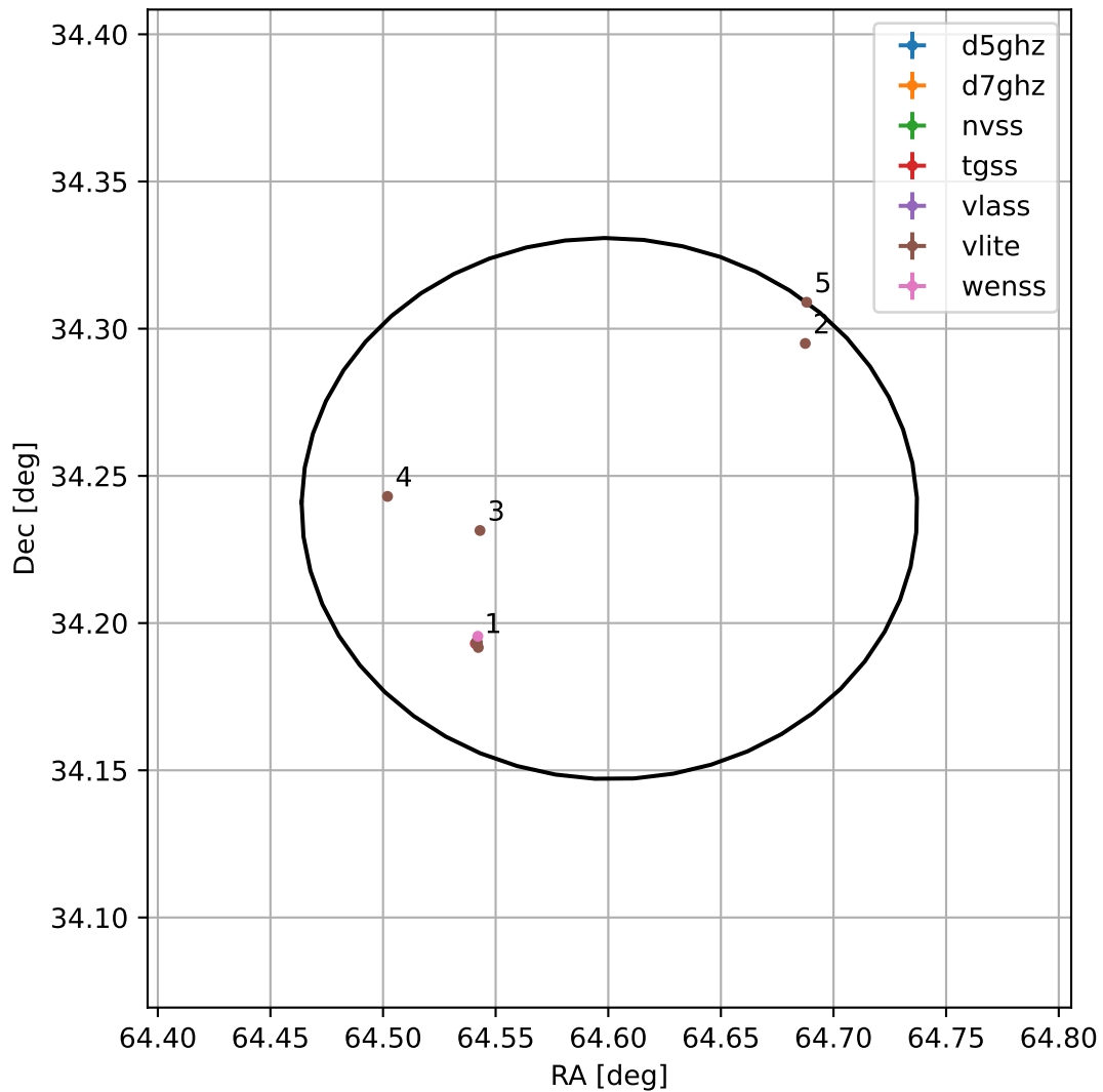
4FGL J0418.4+3414
