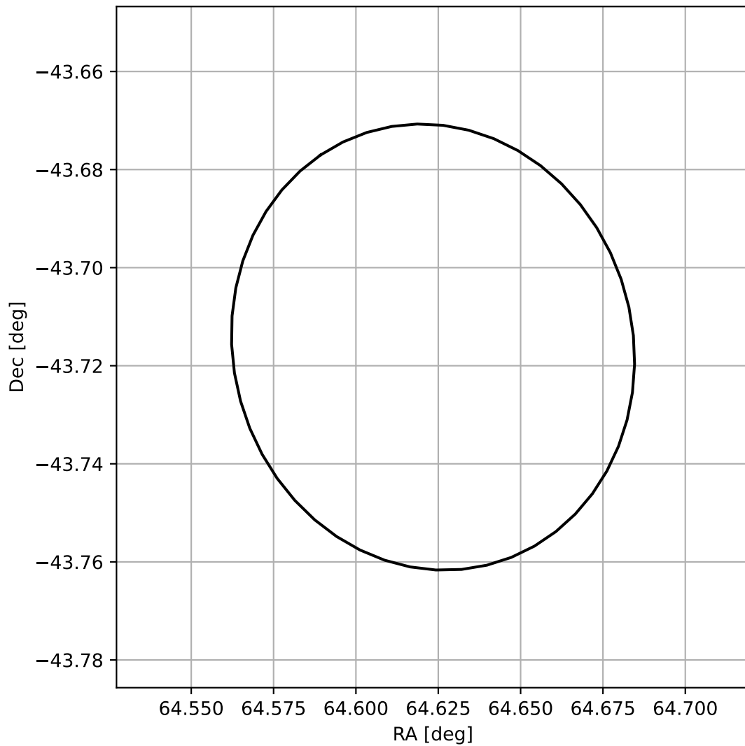
4FGL J0418.4-4342
