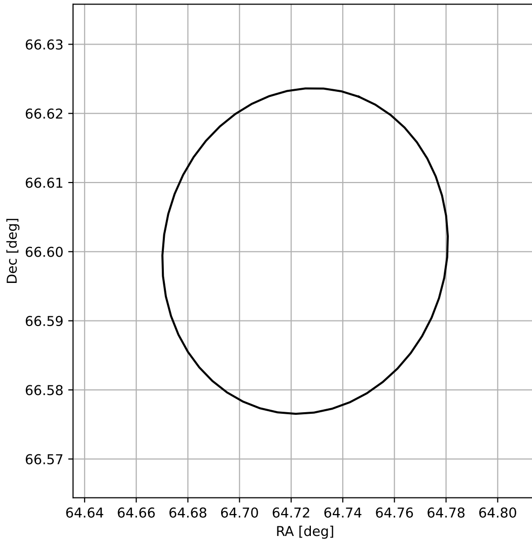
4FGL J0418.9+6636
