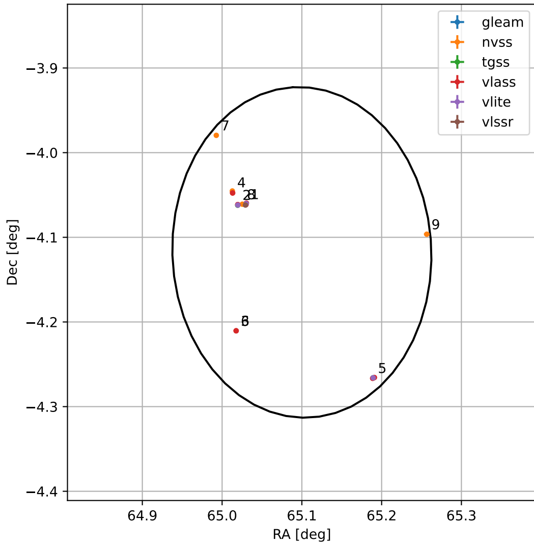
4FGL J0420.3-0407
