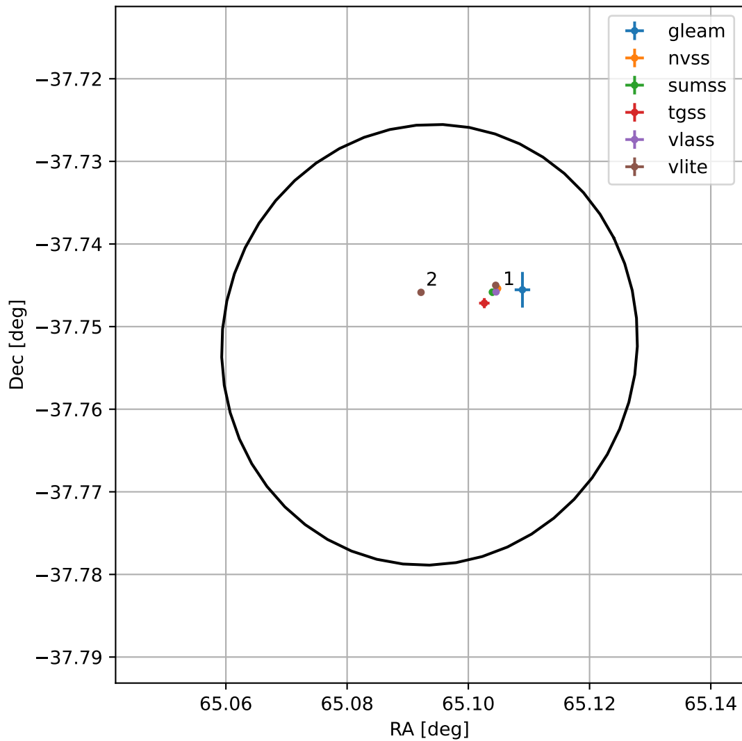
4FGL J0420.3-3745
