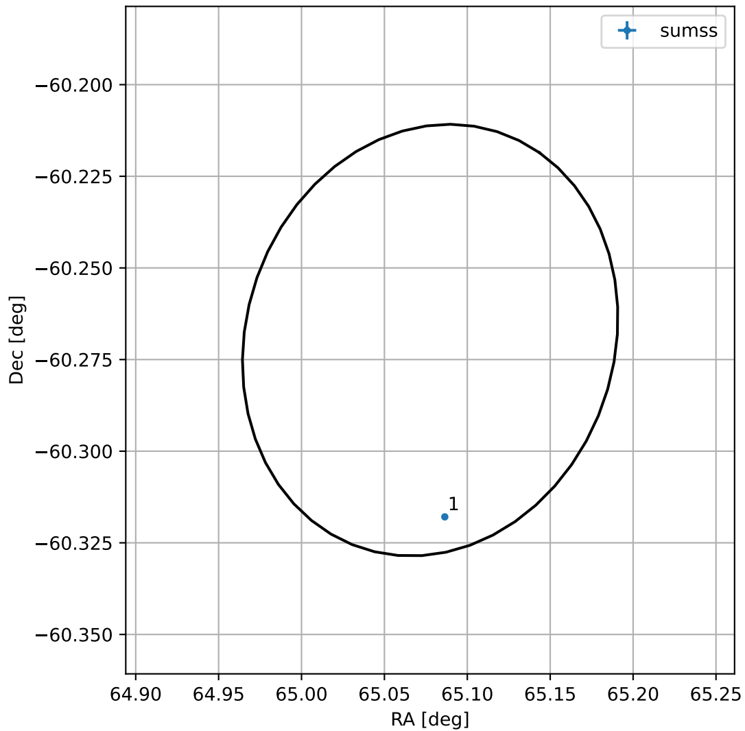
4FGL J0420.3-6016
