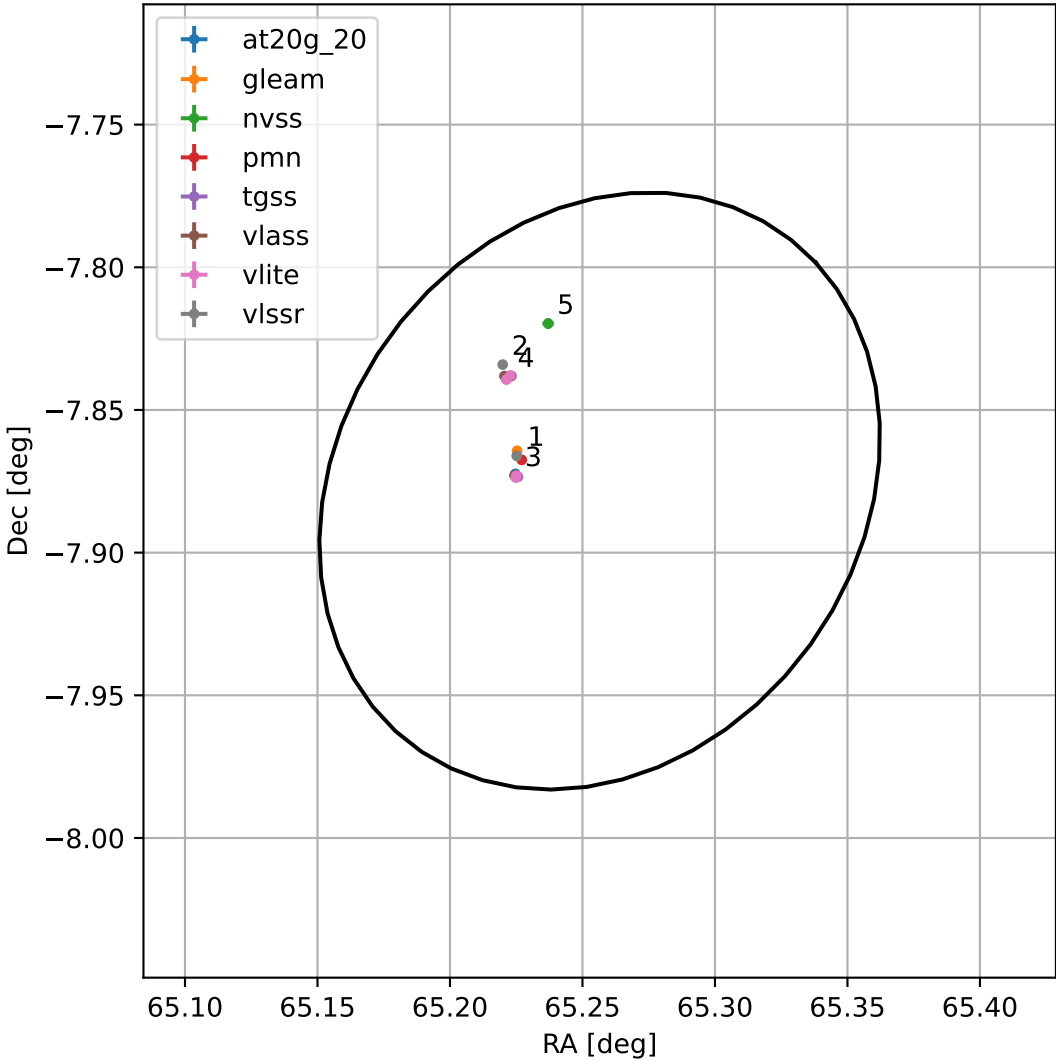
4FGL J0421.0-0752
