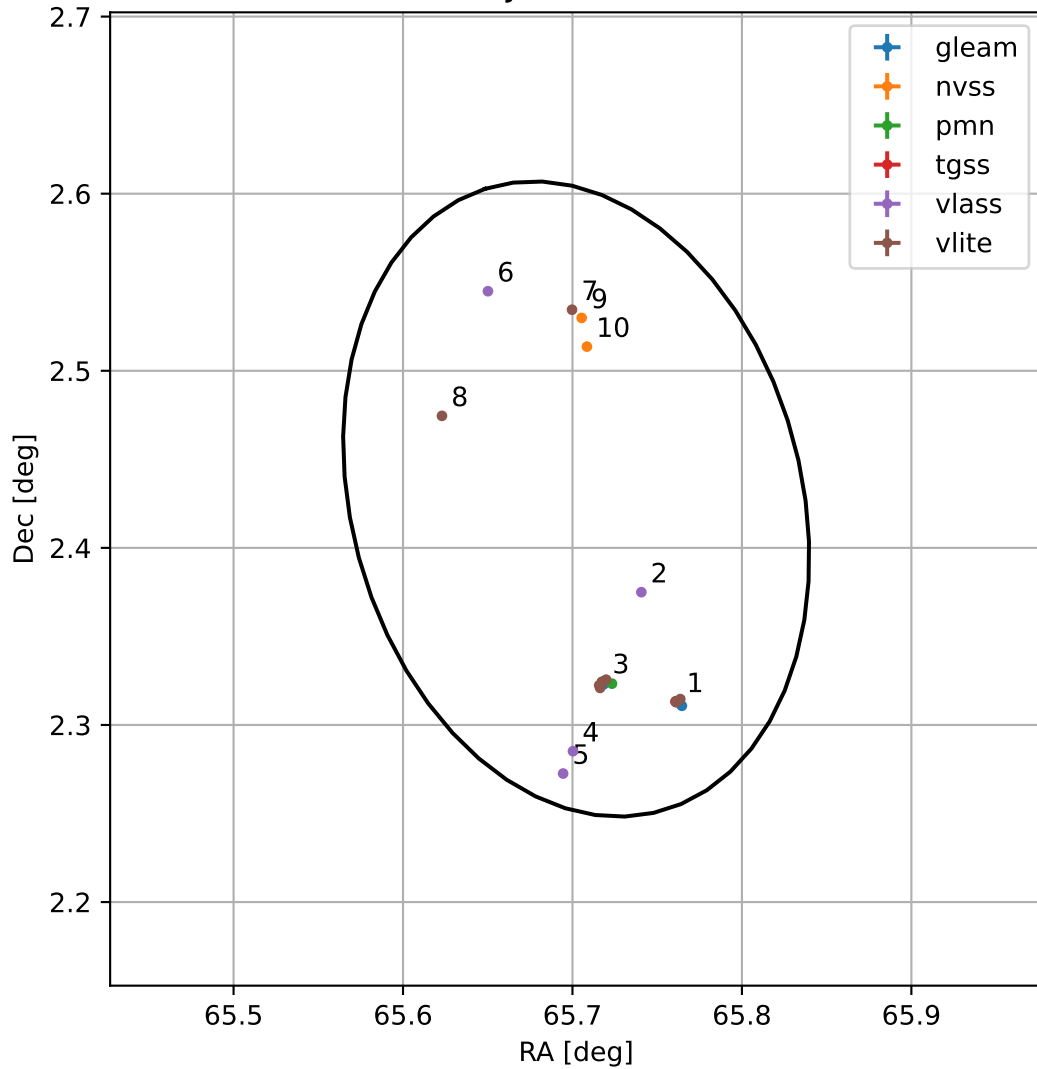
4FGL J0422.8+0225
