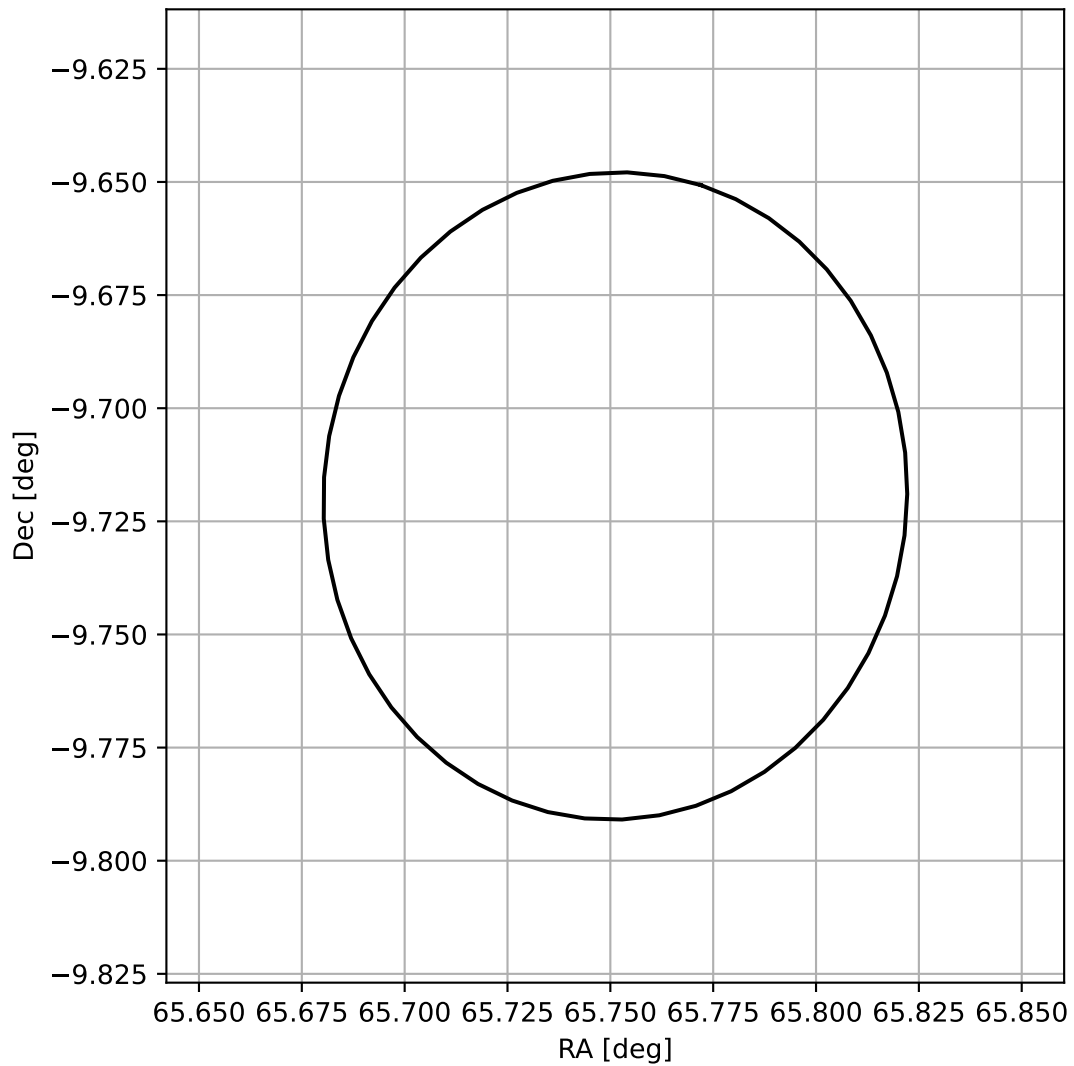
4FGL J0423.0-0943
