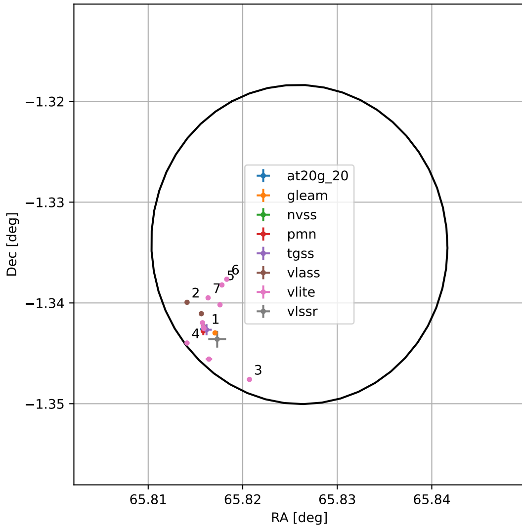
4FGL J0423.3-0120
