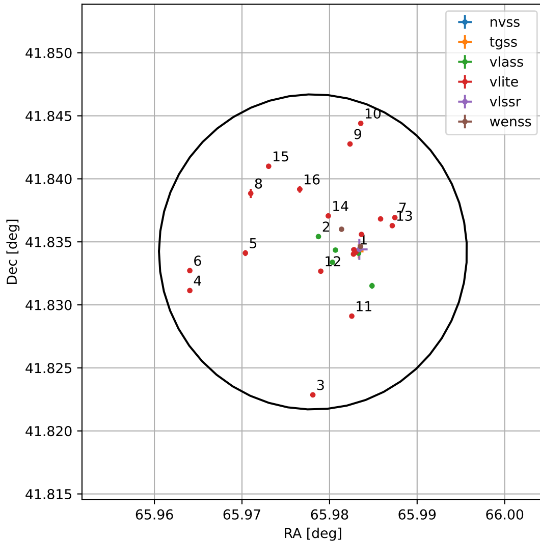
4FGL J0423.9+4150
