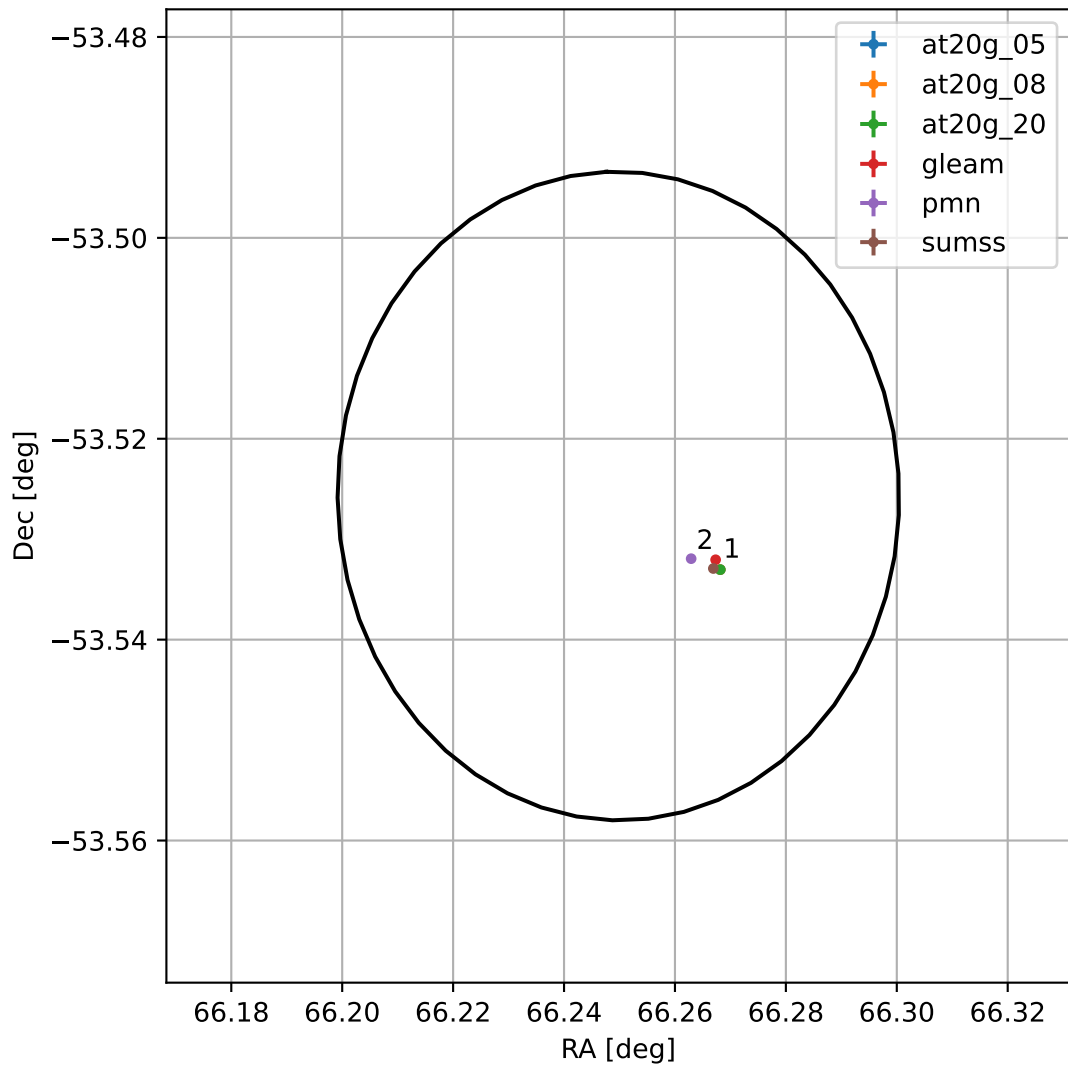
4FGL J0424.9-5331
