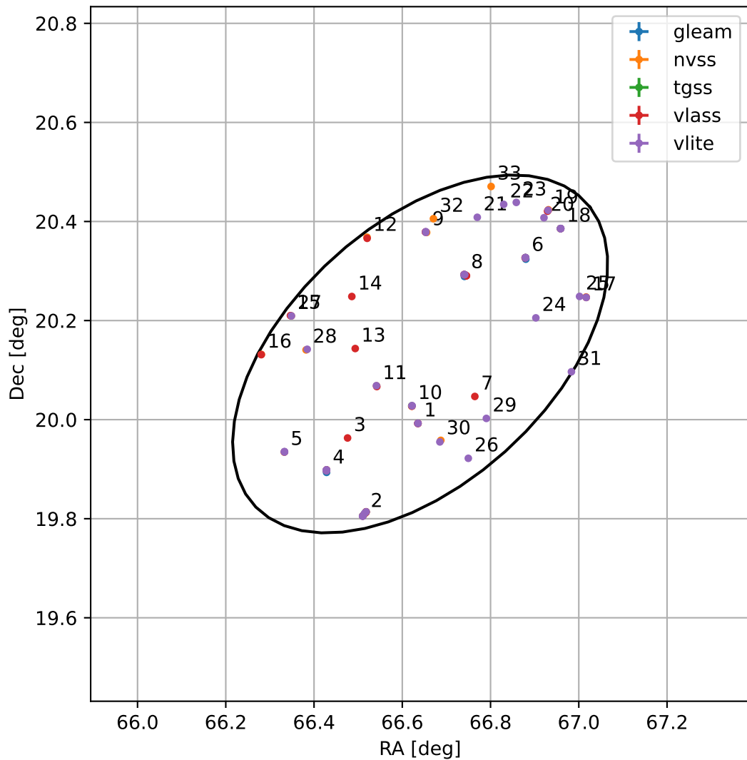
4FGL J0426.5+2007
