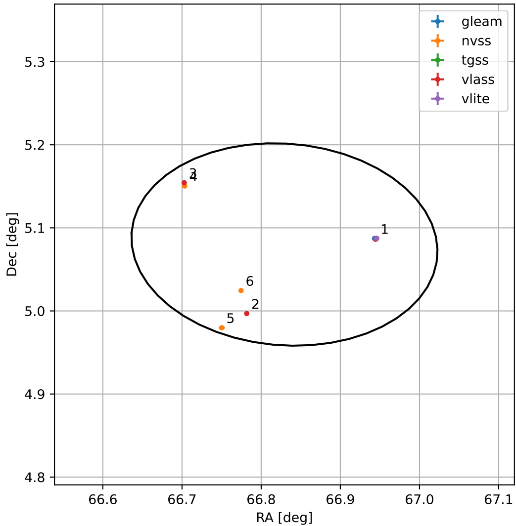
4FGL J0427.3+0504
