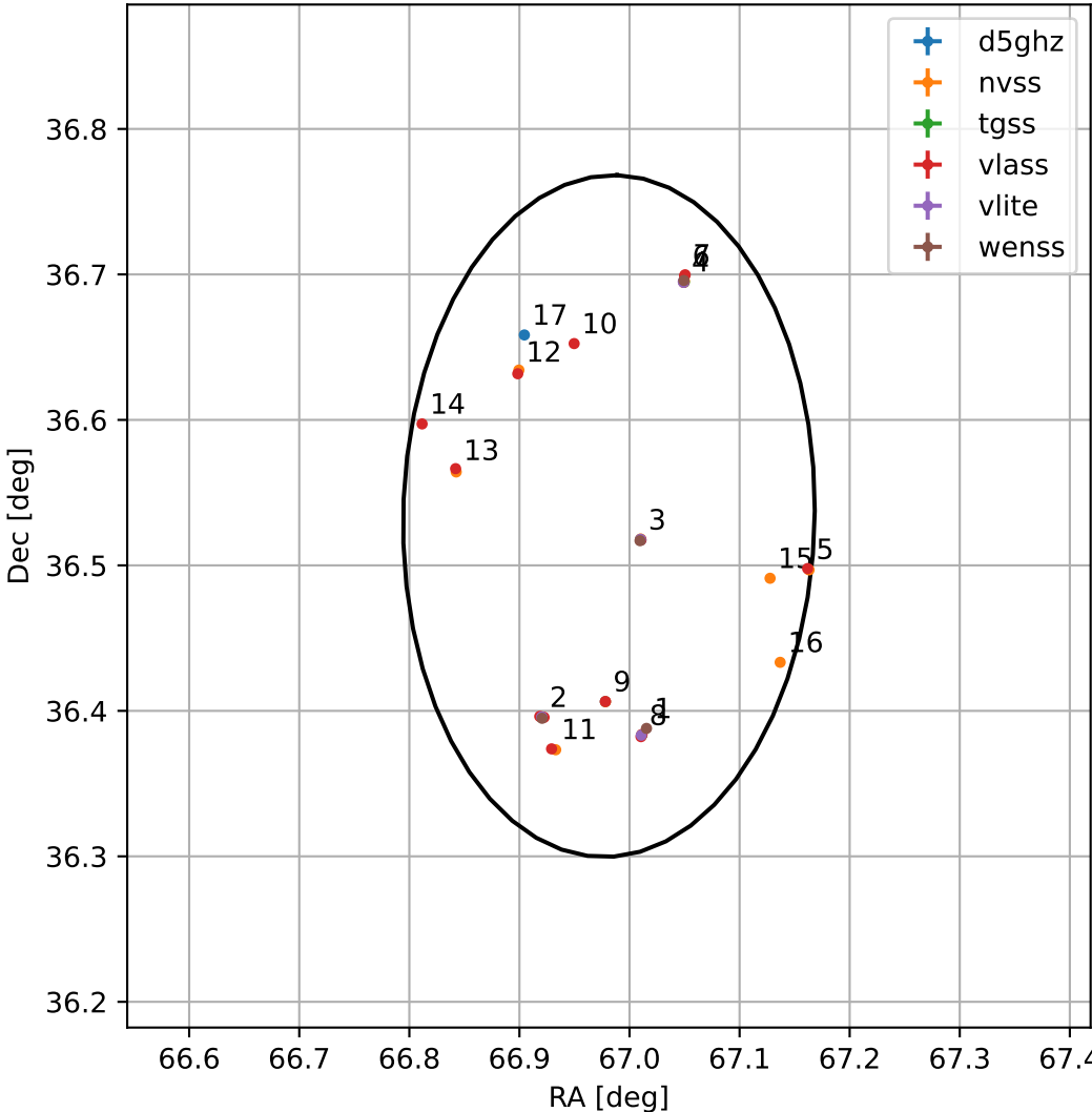
4FGL J0427.9+3632
