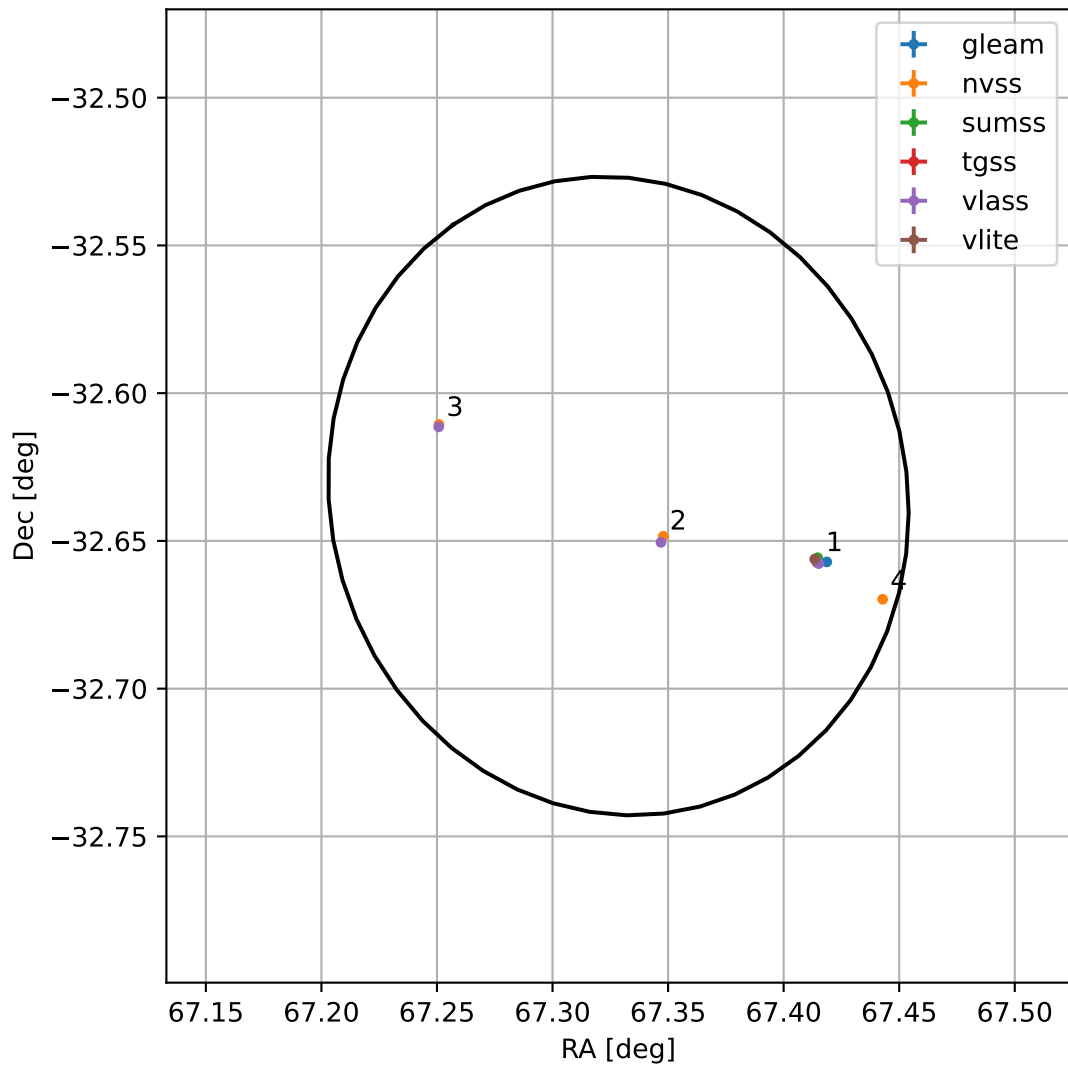
4FGL J0429.3-3238
