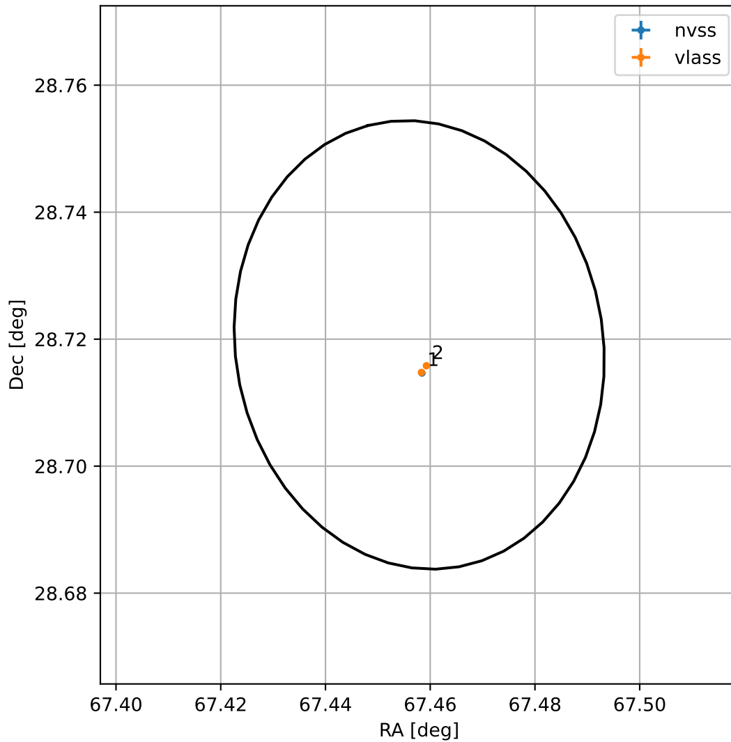
4FGL J0429.8+2843
