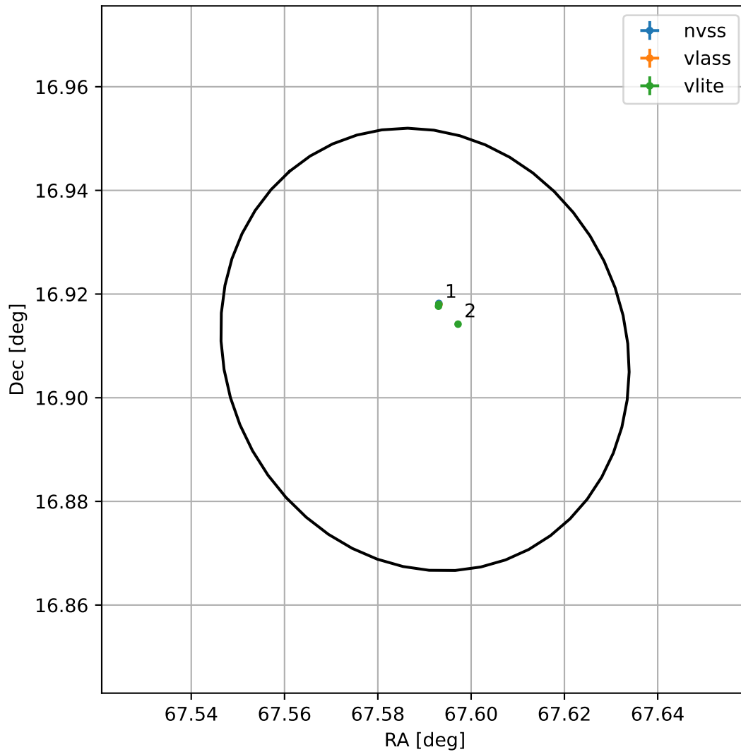
4FGL J0430.3+1654
