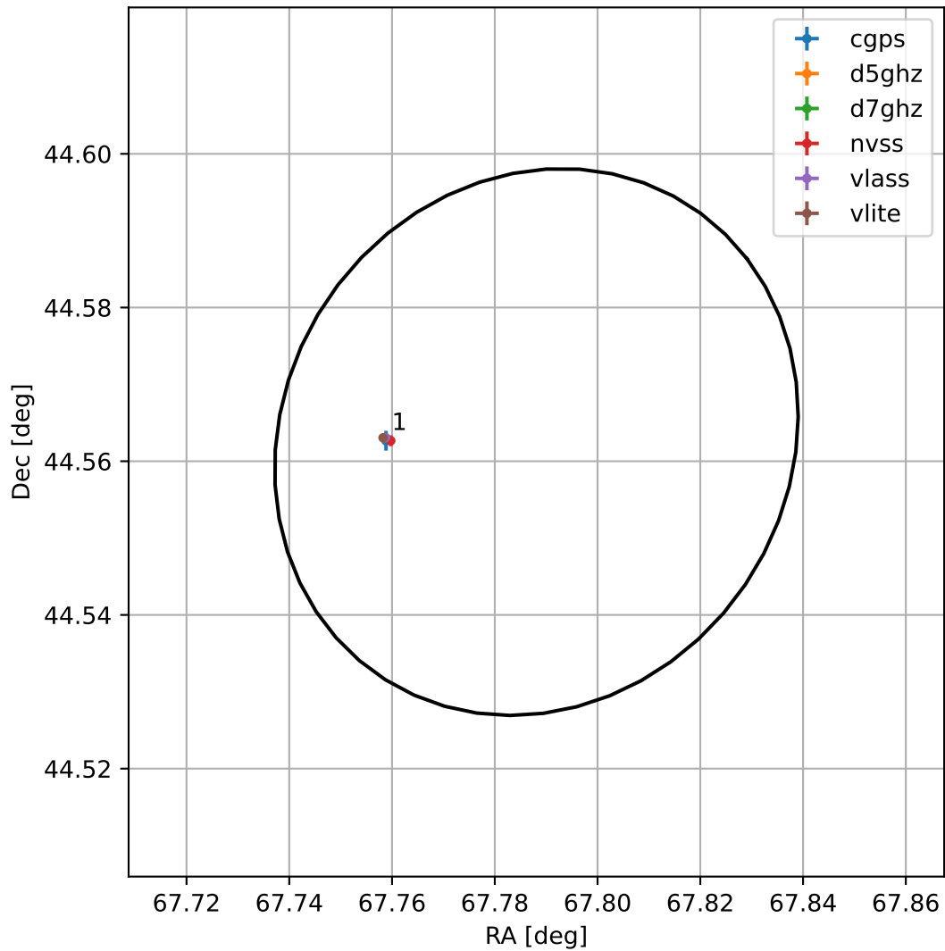
4FGL J0431.1+4433
