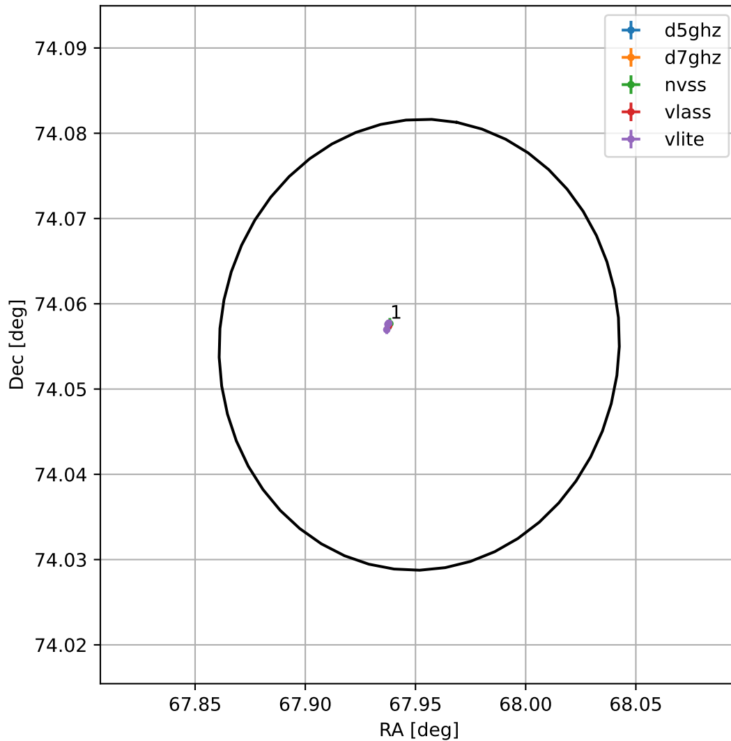
4FGL J0431.8+7403
