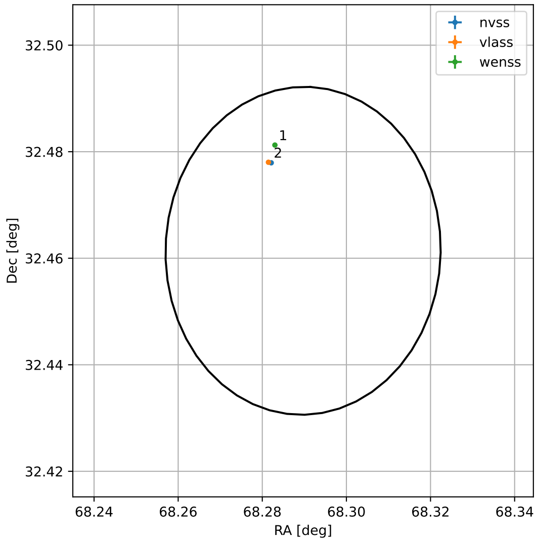
4FGL J0433.1+3227
