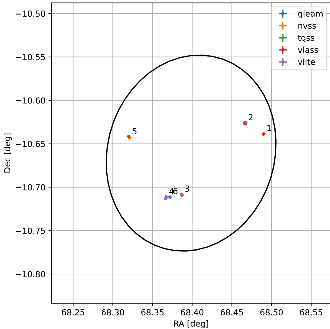
4FGL J0433.5-1039
