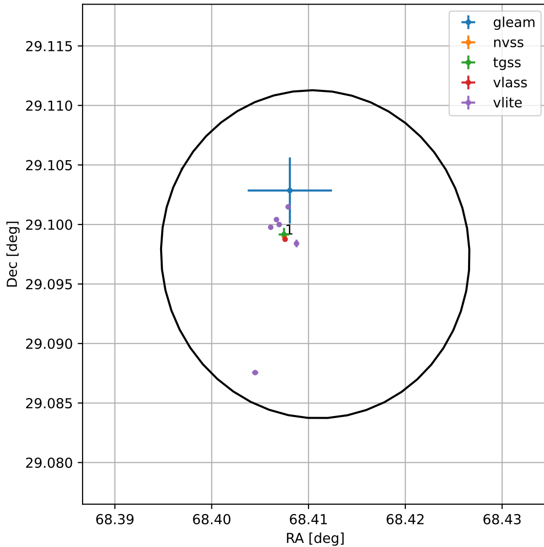
4FGL J0433.6+2905
